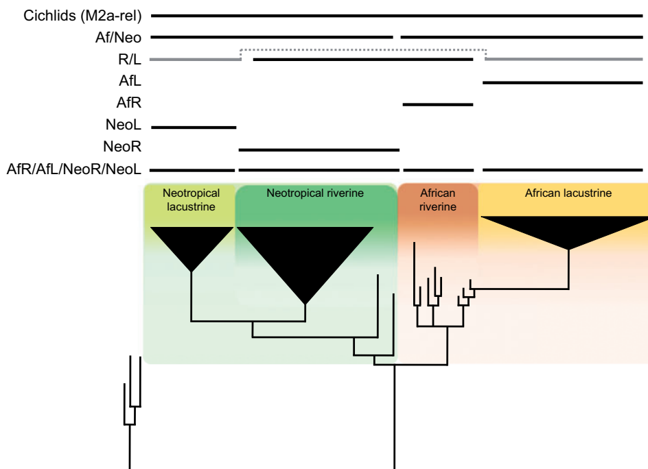
Fig. 2. Simplified representation of the rhodopsin gene tree indicating the a priori partitions among cichlids lineages tested using CmC. Abbreviations refer to riverine (R), lacustrine (L), African (Af), Neotropical (Neo), African riverine (AfR), African lacustrine (AfL), Neotropical riverine (NeoR), and Neotropical lacustrine (NeoL) cichlids. The AfL, AfR, NeoL, and NeoR models contain an implicit second partition that includes all cichlids but those in the depicted partition.
