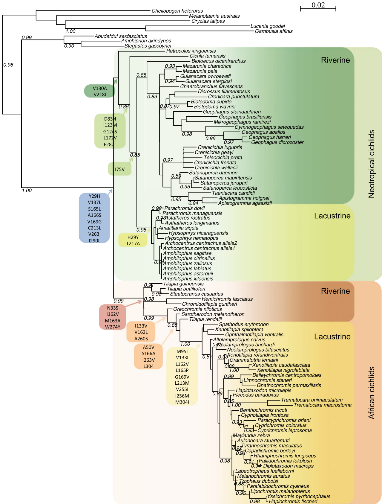
FIG. 1. ML rhodopsin gene tree. The nonparametric aLRT SH-like procedure is only shown when above 0.85. Insets show the amino acid substitution inferred to have occurred in the rhodopsin gene of the ancestor to all cichlids (blue inset), Neotropical cichlids (dark green inset), African cichlids (dark brown inset), Neotropical lacustrine cichlids (light green inset), and African lacustrine cichlids (light brown inset). Ancestral state reconstruction was performed as implemented in PAML.
