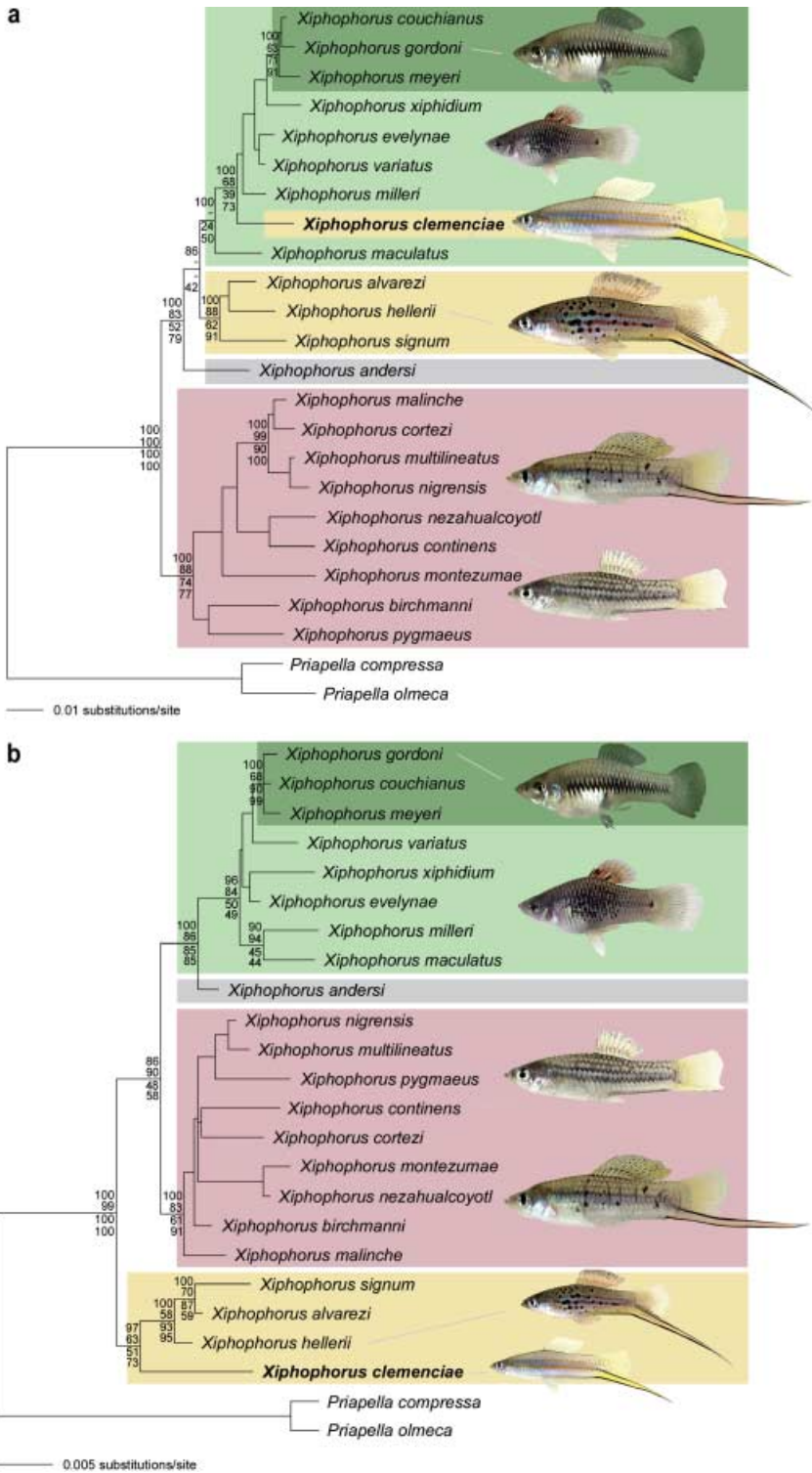
Fig. 2 Phylogeny of all 22 Xiphophorus species using Priapella compressa and Priapella olmeca as outgroup (Meyer et al. 1994). (a) Maximum-likelihood tree based on the complete mitochondrial control region and a segment of the cytochrome b gene (1237 bp). (b) Maximum-likelihood tree based on six nuclear markers (3005 bp). Numbers above the branches are the corresponding Bayesian posterior probabilities and quartet-puzzling values; numbers below the branches represent maximum-parsimony and neighbour-joining bootstrap values. In the mitochondrial phylogeny (a), Xiphophorus clemenciae is nested among the southern platyfish; in the nuclear tree (b) it is grouped together with the southern swordtails instead.
