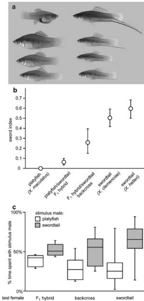
Fig. 3 Laboratory crosses between Xiphophorus maculatus females and males of the swordtail Xiphophorus hellerii . (a) On the left side are females; on the right sides, males. The two fish in the top row are a X. maculatus female and a male swordtail X. hellerii . Below are BC 1 hybrid females and males. (b) Sword index (sword length/standard length) of male platyfish ( X. maculatus ), (female) platyfish/swordtail ( X. hellerii ) F 1 hybrids ( N = 14 ), backcross hybrids from F 1 hybrid females mated with swordtail males ( X. hellerii ) ( N = 108 ), and swordtail ( X. hellerii ) males ( N = 32 ), for comparison the sword index of Xiphophorus clemenciae males ( N = 17 ) is shown as well. Bars show standard deviation. (c) To analyse the preference of platyfish/swordtail F 1 hybrid females, standard visual choice tests were performed. The box plots depict the preferences of platy/swordtail F 1 hybrid females, backcross hybrid females from F 1 females mated with swordtails, and swordtail females. The bar represents the median of the time spent with the stimulus male, the box characterizes the 25% and 75% values, respectively. The whiskers describe the 10% and 90% values, respectively. There is tendency of F 1 hybrid females towards a preference for swordtail males over platy males although not statistically significant ( N = 9 , z = -1.96 , P = 0.0499 ). Backcross females from matings of F 1 hybrid females with swordtail males significantly preferred the swordtail males over platy males ( N = 28 , z = -2.715 , P = 0.0066 ). Swordtail females preferred the conspecific males over the males of the platyfish ( N = 28 , z = -2.859 , P = 0.0043 ).
