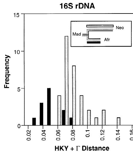
Fig. 4. Frequency distribution of genetic distances among cichlids (HKY + \Gamma distances). Path lengths across the ME tree from the most common recent ancestor (MRCA; see insert ) to Neotropical genera (Neo; hatched bars ) and African genera (Afr; solid bars ). Mad, Madagascar/Indian cichlids. To minimize the effect of nonindependence among distances, a single representative of each Neotropical genus was used when more than one species per genus was available. A slower rate is inferred for African cichlids based on the shorter path length from Madagascar/Indian to African cichlids than to Neotropical cichlids.
