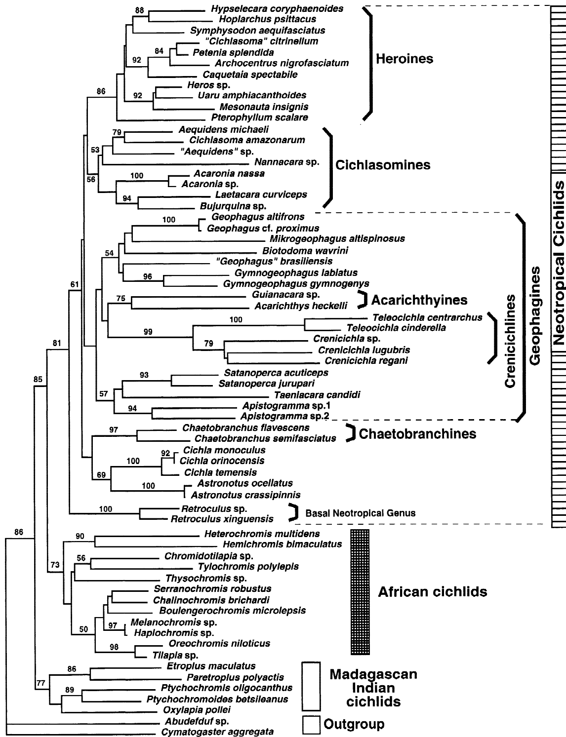
Fig. 3. ME tree obtained using HKY + \Gamma distances (ME score = 3.75, T ratio = 2.45, Pinvar = 0.39, \Gamma shape = 0.67). Numbers above branches are bootstrap values (only values above 50 are shown). Highlighted branches identify the highest rates of evolution as suggested by relative rates tests; see text and Fig. 4.
