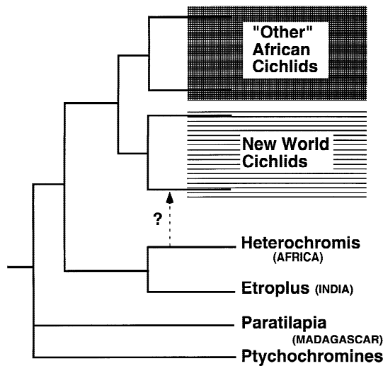
Fig. 1. Phylogenetic relationships of the major groups of cichlid fish based on morphological characters according to Stiassny (1991) and supported (in part) by nuclear molecular markers, except for the controversial position of the African genus Heterochromis . While Stiassny (1991) suggested a close relationship of Heterochromis with etroplines, Kullander (1998) placed it among basal Neotropical cichlids.
