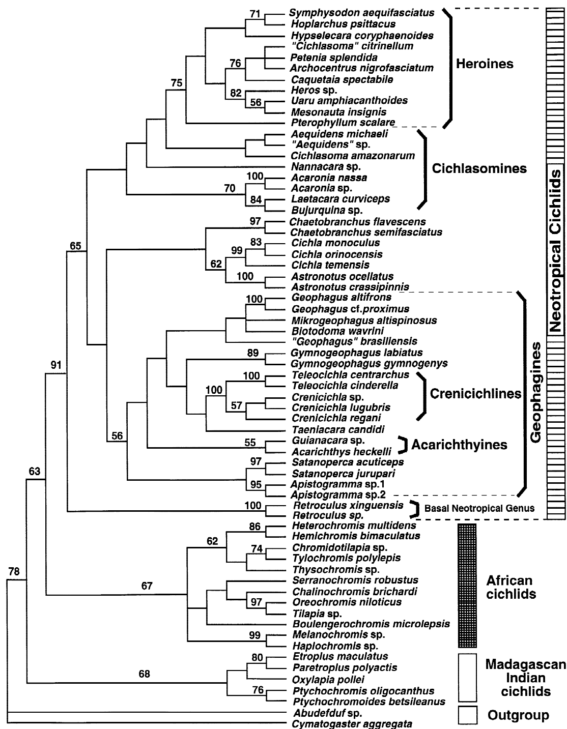
Fig. 2. Strict consensus of eight MP trees. Numbers above branches are bootstrap values (only values above 50 are shown).
